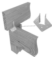
Typical RT15-TZ installation
