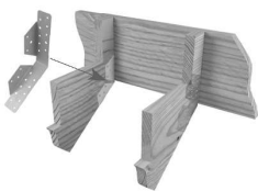
Typical CSH-TZ installation
