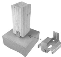
Typical PAF-TZ installation
