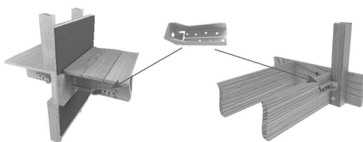
Typical DTB-TZ installations
